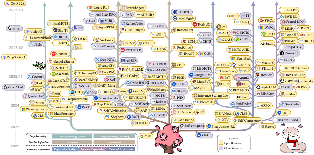
Figure 1: Evolution of selected Long CoT over the past three years, where colored branches represent different characteristics: deep reasoning , feasible reflection , and extensive exploration . Each characteristic is further divided into key areas: Deep reasoning includes its format and learning methods. Feasible reflection focuses on feedback and refinement techniques during reflection process as optimization strategies. Extensive exploration addresses scaling, internal, and external exploration as key improvements to Long CoT.
